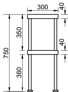
SIDE ELEVATION
